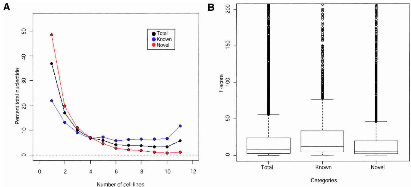
Figure 5 Analysis of the expression and variance of known and novel transcription across all 11 cell lines. (A) Expression of known and novel transcription from 11 cell lines by the percentage of total nucleotides within the total (black), known (blue), and novel (red) transfrags according to the number of cell lines expressing that transfrag. (B) Estimation of the degree of differential expression across the 11 cell lines. An F -statistic was calculated for each transfrag by the variance of the average pseudo-median value in each transfrag between cell lines divided by the average of the within cell line variation of the pseudo-median value in that transfrag.
