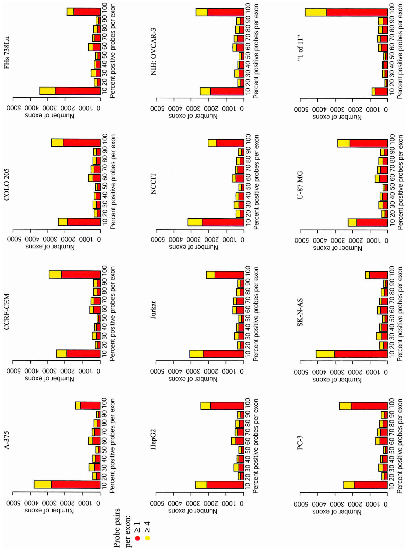
Figure 3 Distribution of positive probes in exons. The distribution of the percent of positive probes in exons is plotted by cell line as well as for the "1 of 11" map. The red bars represent all interrogated exons, and the yellow bars represent exons that contain four or more interrogating probe pairs.
